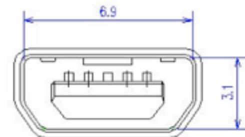
mini-AB connector
