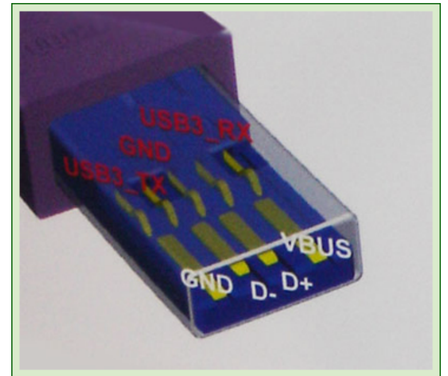
Type A USB 3.0 connector Upstream (Host, Hub)
