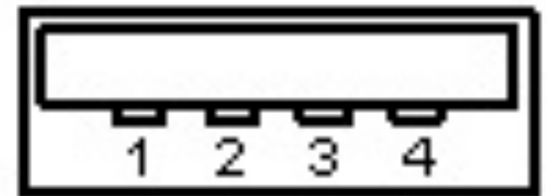
Type A USB connector Upstream (Host, Hub)
