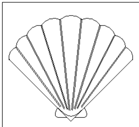
Original Texture
