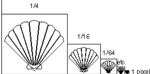
Pre-Filtered Images
