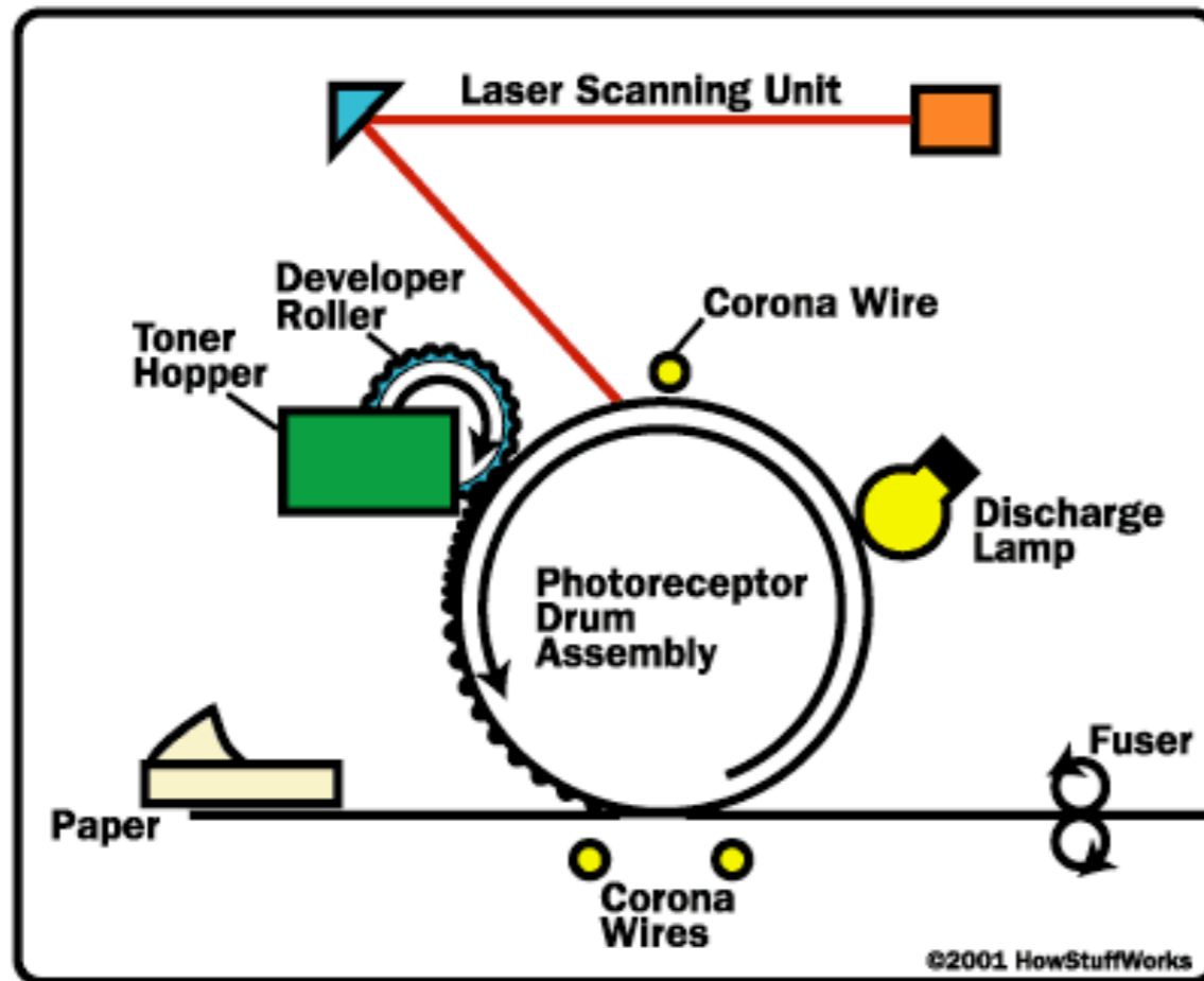
The basic components of a laser printer
